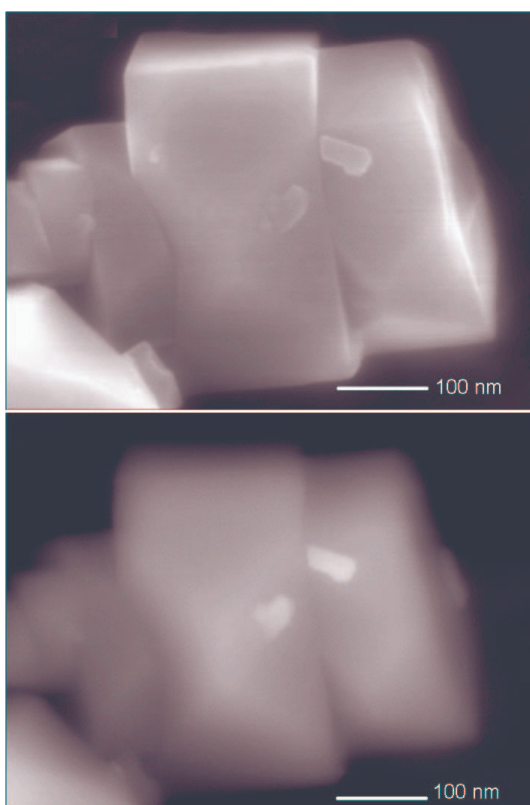
Figure 3: SEI and BEI taken at 200 kx. The bar corresponds to 100 nm. The particles over the zeolite blocks are Co particles of around 25 nm and are noticed in the BEI micrograph.
