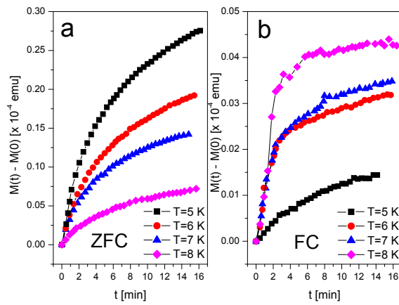
Figure 9: M vs. t for different temperatures. (a) After ZFC in mode (i). (b) After FC in mode (iii).
