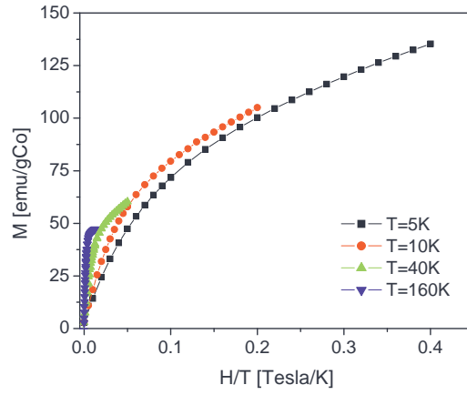
Figure 8: M vs. H/T . No universal curve is found, due to several contributions to the magnetization.
