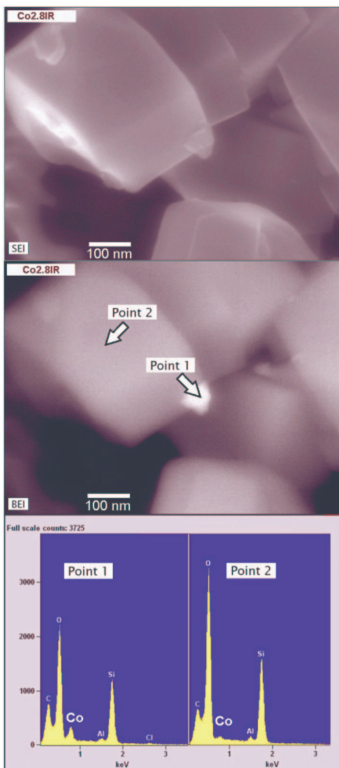
Figure 2: SEI (top) and BEI (middle) taken at 150 kx. The bar corresponds to 100 nm. The EDS spectra at the bottom correspond to Points 1 and 2, respectively, indicated with white arrows in the BEI micrograph. The particle indicated in Point 1 is a Co particle and has a size of 60 nm.
