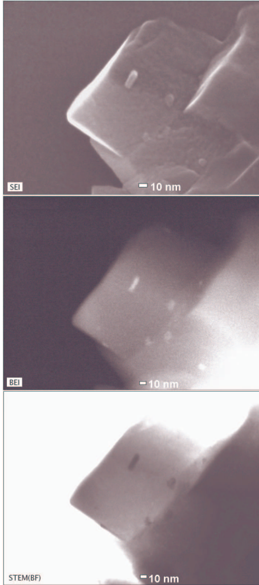
Figure 4: SEI and BEI taken at 300 kx (top and middle). The bar corresponds to 10 nm. The bottom image is a scanning transmission electron micrograph (STEM) of the same portion as shown above.
