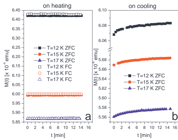
Figure 10: M vs. t for sample Co 2.8 IR, for different temperatures, reached on heating (modes (ii) and (iv) in part a) and on cooling (mode (i) in part b).
