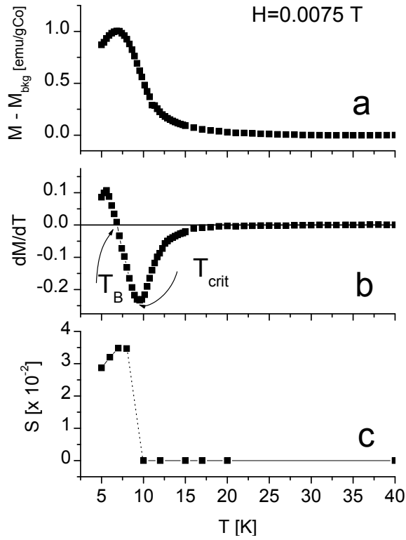
Figure 11: M(T) vs. T and dM/dT vs. T , ZFC curve. a) M(T) corresponding to the low temperature peak after background subtraction. b) dM/dT , where the blocking temperature T_B is defined as the temperature where dM/dT = 0 and the temperature T_{\text{crit}} where d^2M/dT^2 = 0 . c) Viscosity constant S(T) .
