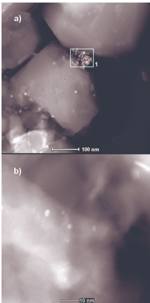
Figure 5: a) STEM image of a cluster of small Co particles. Bar=100 nm. b) STEM image (acquired with HAADF detector) of the smaller features of the studied sample. Particles smaller than 10 nm are noticed on the surface. Bar=10 nm.
