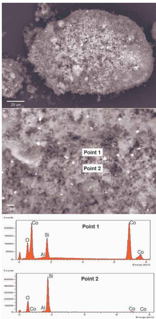
Figure 1: Low magnification SEM micrographs. Top: 1.5 kx; the bar corresponds to 20 \mu\text{m} . Middle: 6 kx; the bar corresponds to 2 \mu\text{m} . The bright spots on the zeolite surface are Co particles; Point 1 marks a bright spot and Point 2 marks a dark zone. Bottom: EDS spectra corresponding to Point 1 and Point 2. Both the characteristic lines of Co (very intense) and the matrix are clearly seen in Point 1 spectrum, while the other shows the characteristic lines of the matrix and very small peaks of Co energies.
