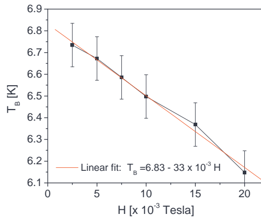
Figure 7: Blocking temperature T_B as function of the applied field H .
