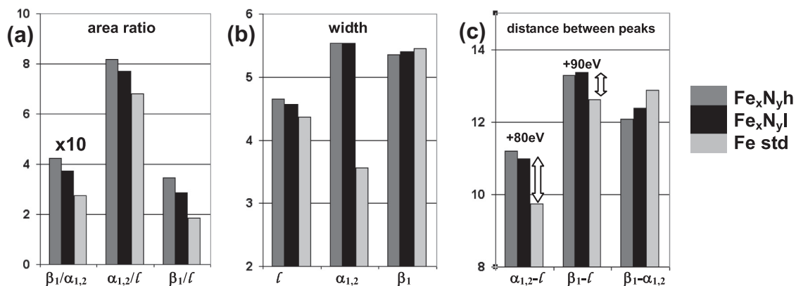
Fig. 4. Comparison of (a) the peak area ratios, (b) the peak widths, and (c) the distance distances between indicated peaks in the nitrated samples and the Fe standard. The chemical shifts of the L\alpha_{1,2} and L\beta_1 peaks are indicated with block arrows in (c).
