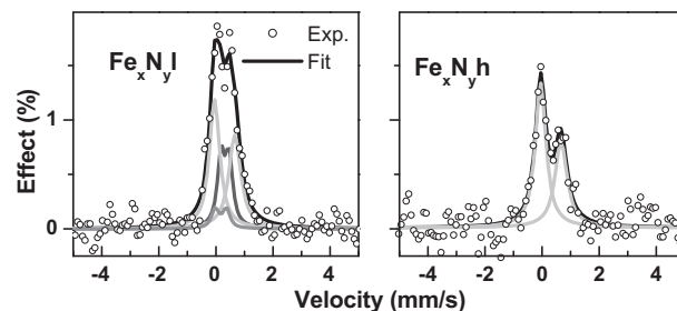
Fig. 1. CEMS of the nitrided samples. Open symbols are the experimental data, black solid lines are the sum of the partial spectra (see Section 3.4).
