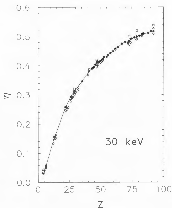
Figure 2. Backscattering coefficient versus atomic number Z for 30 keV electrons at normal incidence. Open symbols are experimental data from different sources: Hunger and Kuchler (1979), diamonds; Drescher et al. (1970), up triangles; Neubert and Rogaschewski (1980), squares. Solid circles represent results from PENELOPE, joined by straight segments for visual aid, the error bars (three standard deviations) are of the same size as the symbols.
