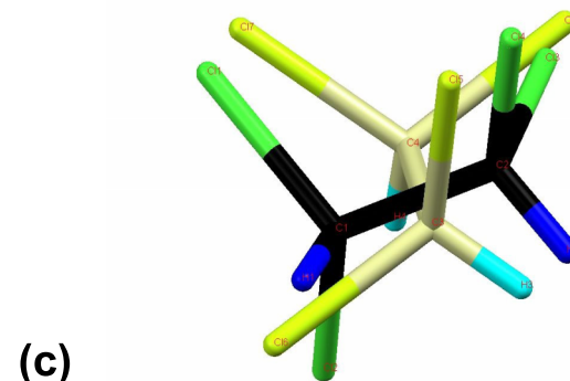
FIG. 4. Carbon (a) and selected chlorine (b) coordinates of a TCE molecule during 10 ns of NVT molecular dynamics simulations covering a dynamic transition to and from a high-energy orientational state. (c) Relative orientations of a TCE molecule in the high-energy orientation (yellow) as compared to the ground-state orientation (black).
