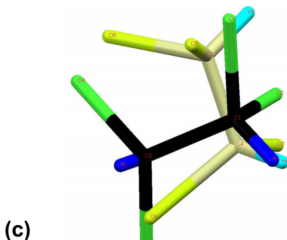
FIG. 3. Carbon (a) and selected chlorine (b) coordinates of a TCE molecule during 1.5 ns of NVT molecular dynamics simulations covering the 180^\circ flip about the molecular symmetry axis. (c) Relative orientation of the intermediate state attained during such reorientational motion (yellow) with respect to the initial/final state (black).
