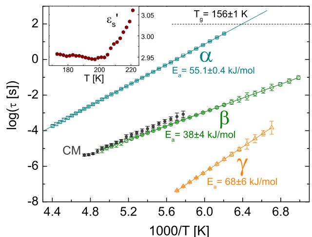
FIG. 2. Arrhenius plot of the characteristic times of all three relaxation processes ( \alpha , \beta , and \gamma ) observed in TCE (open markers with error bars). Continuous lines are fits with the Arrhenius Eq. (2), and the dashed line indicates the glass transition temperature of the \alpha process. Filled circles with error bars indicate the predicted relaxation time of the Johari-Goldstein precursor according to the Coupling Model (CM) (Eq. (3), see the text for more details). Inset: plot of the static permittivity \epsilon_s as a function of temperature.
