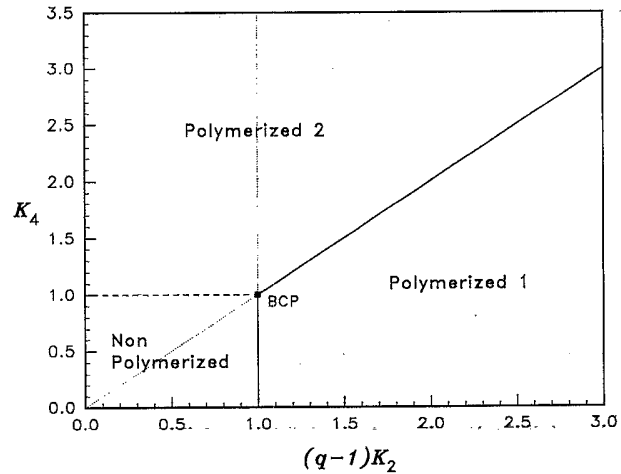
FIG. 3. K_4 against (q-1)K_2 phase diagram for the Bethe lattice with coordination number q = 4 . The full lines represent second order transitions and the dashed line locates the first order transitions. The stability (spinodals) curves are also shown (dotted lines). The critical lines end in a bicritical point (BCP).
