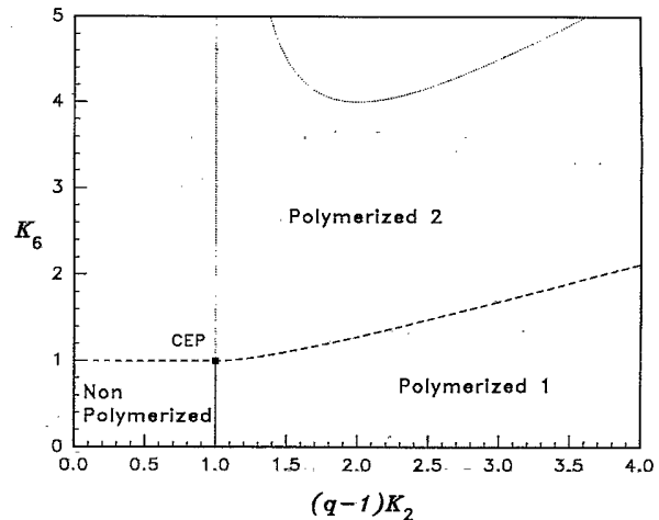
FIG. 6. K_6 against (q-1)K_2 phase diagram for a q = 6 Bethe lattice, showing the second order line (full line), the first order curve (dashed line), and the spinodal lines (dotted lines). The critical line ends in a critical end point (CEP).
