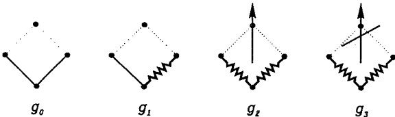
FIG. 9. Root configurations associated with the three partial partition functions of subtrees on a Husimi tree with q = 4 . Straight lines represent empty bonds, zigzag lines represent polymer bonds, and dotted lines may be occupied by a polymer bond or not. The arrow means that the polymer network is connected to the boundary and the crossed arrow means that the polymer does not reach the boundary.
