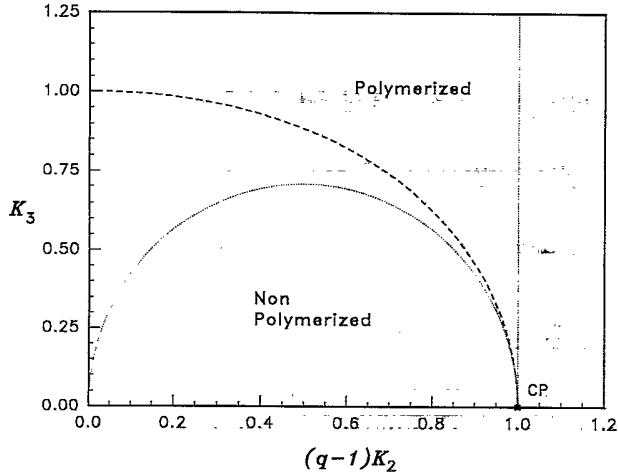
FIG. 4. K_3 against (q-1)K_2 phase diagram for a q = 3 Bethe lattice, showing the first order curve (dashed line) and the spinodal lines (dotted lines), as well as the critical point (CP) corresponding to the SAW limit K_3 = 0 .
