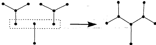
FIG. 1. Construction of a ( q = 3 , M = 3 ) subtree with q = 3 and M = 3 generations by attaching q - 1 = 2 subtrees with q = 3 and M = 2 generations.
