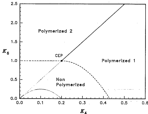
FIG. 7. K_6 against K_4 phase diagram for the q = 6 Bethe lattice, showing the second order line (full line), the first order curve (broken line), and the spinodal lines (dotted lines). The critical line ends in a critical end point (CEP).
