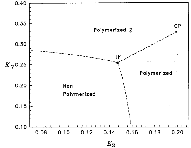
FIG. 8. K_7 against K_3 phase diagram for the q = 9 Bethe lattice, showing three first order lines (dashed line) joined in a triple point (TP). The polymerized 1-polymerized 2 first order line ends in a critical point (CP).
