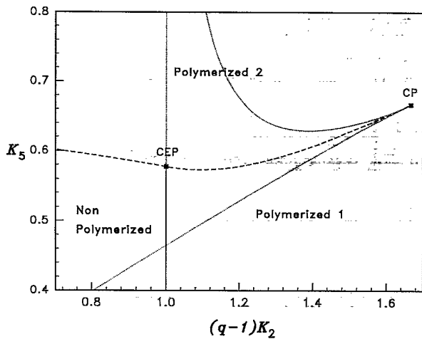
FIG. 5. K_5 against K_2 phase diagram for the q = 6 Bethe lattice, showing the second order line (full line), the first order curve (dashed line), and the spinodal lines (dotted lines). The critical line ends in a critical end point (CEP) and the first order line ends in a critical point (CP).
