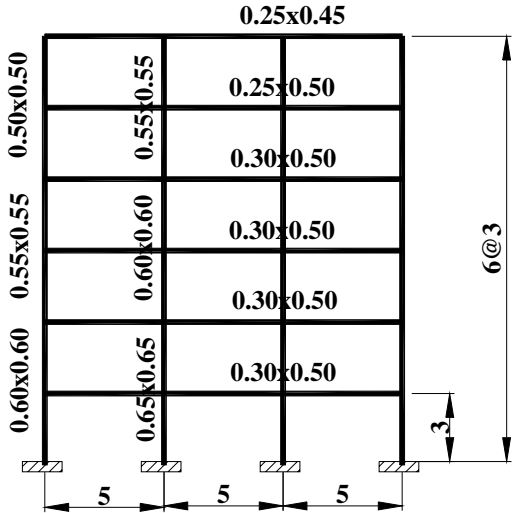
Figure 5. Reinforced concrete 2D frame structure.
