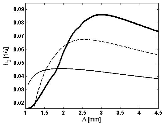
Figure 4. Instantaneous damping coefficient vs instantaneous amplitude. Cases: — 1, - - - 2, ——— 3.
