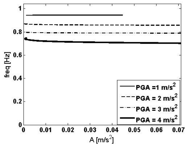
Figure 7. Instantaneous undamped fundamental frequency vs. instantaneous vibration amplitude.
