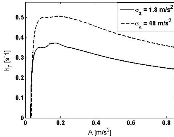
Figure 17. Instantaneous damping coefficient vs instantaneous amplitude of vibrations.
