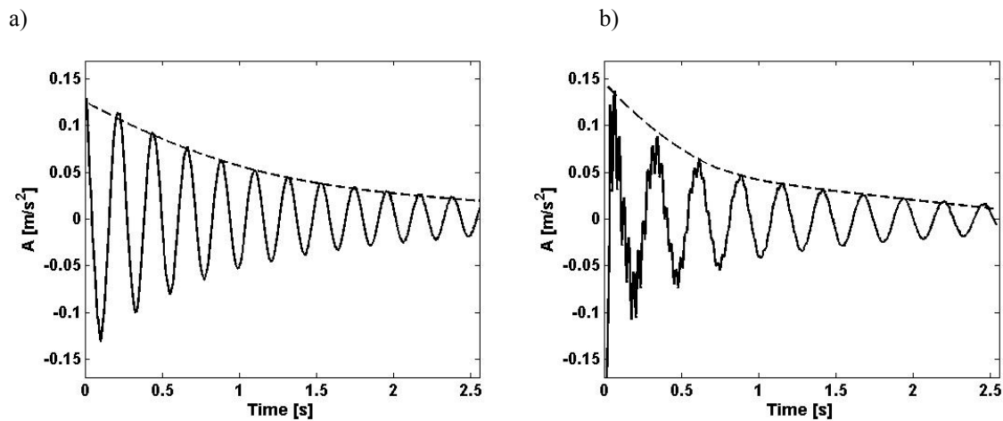
Figure 11. Free vibration response and his envelope after: (a) Test after load step 1 and (b) test after load step 5. (Palazzo, 2000).
