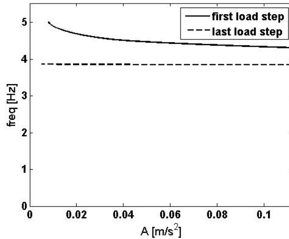
Figure 12. Instantaneous undamped fundamental frequency vs instantaneous amplitude of vibrations.
