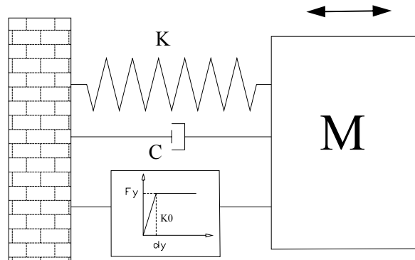
Figure 1. Non linear (bilinear) oscillator (Cases 1 to 3).
