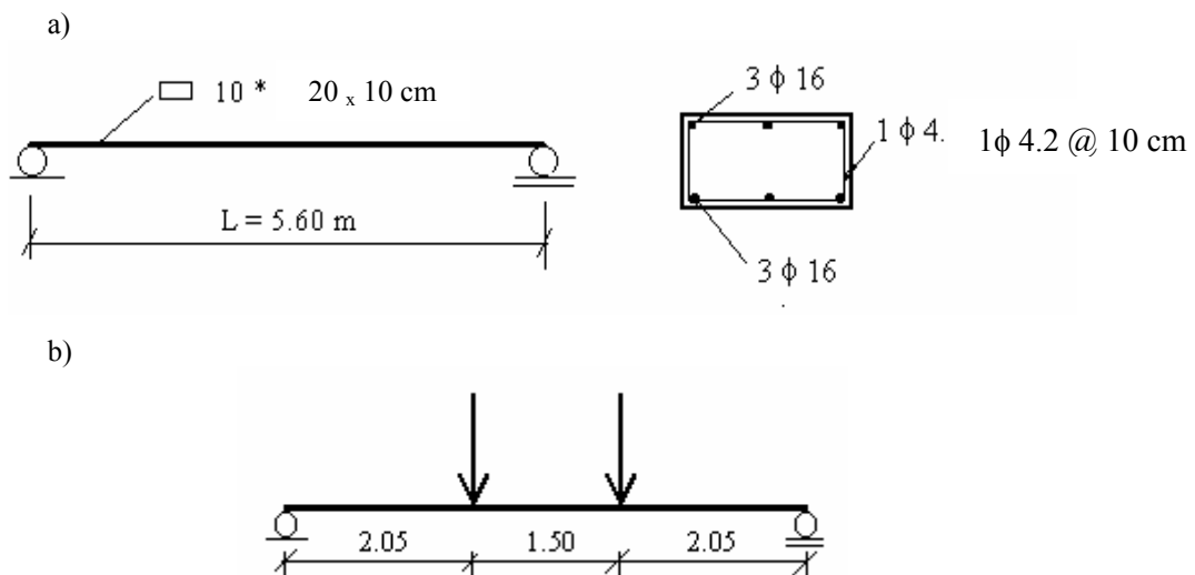
Figure 9 (a) Sketch of reinforced concrete simply supported beam tested (b) load location.
