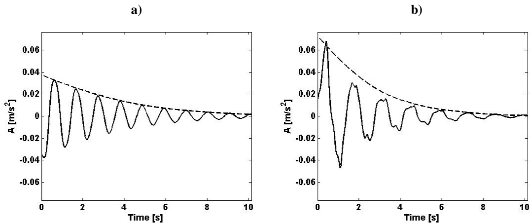
Figure 6. Free vibration response and envelope. (a) first and (b) ultimate degree of damage of 2D Frame Structure.
