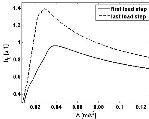
Figure 13. Instantaneous damping coefficient vs instantaneous amplitude of vibrations.
